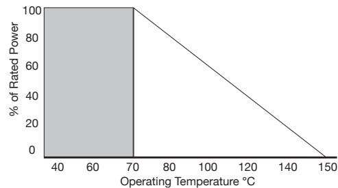
Derating Curve
